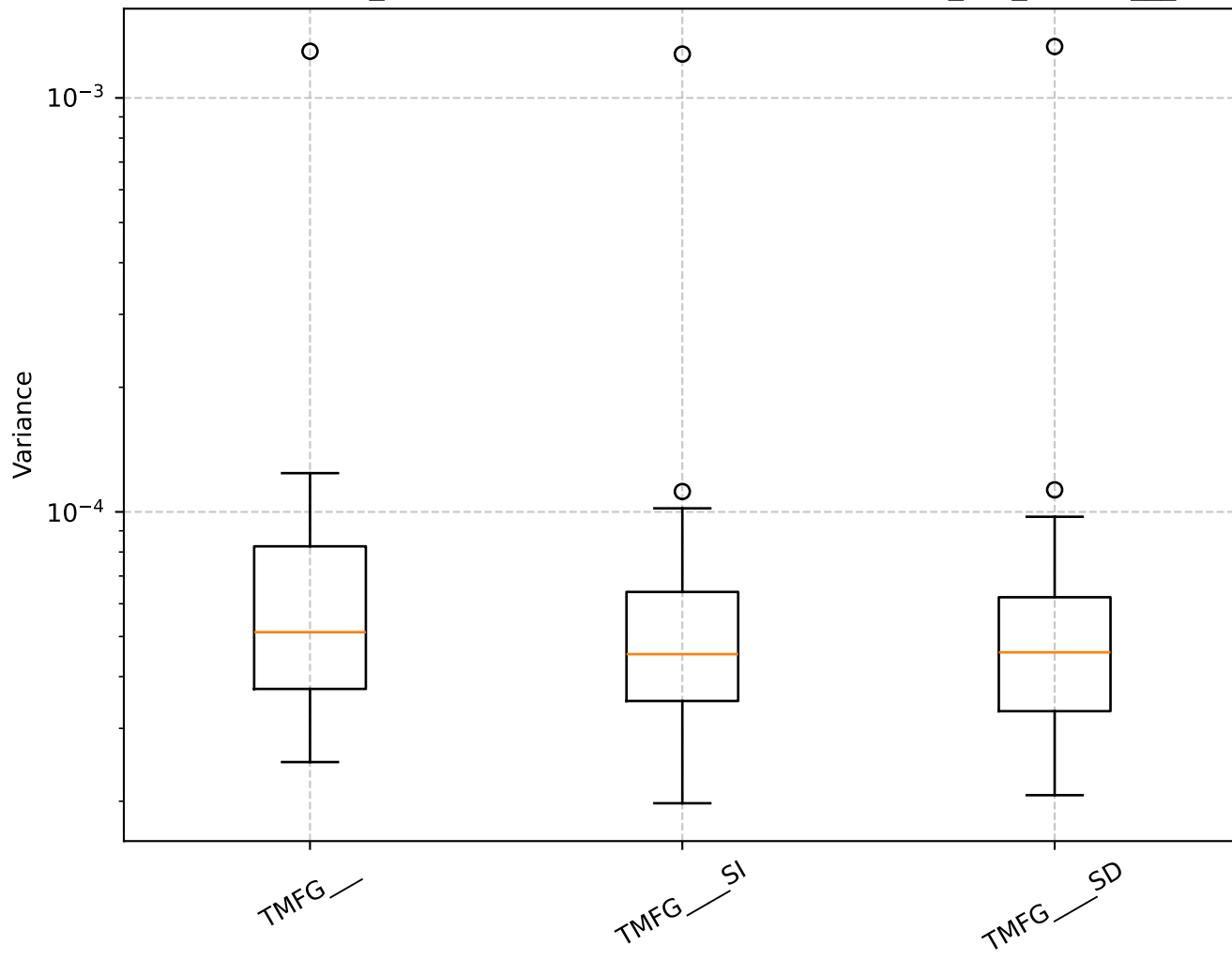
Q=0.51, len_rolling=100: Shrinkage Box Plot - min_var_, TMFG__
