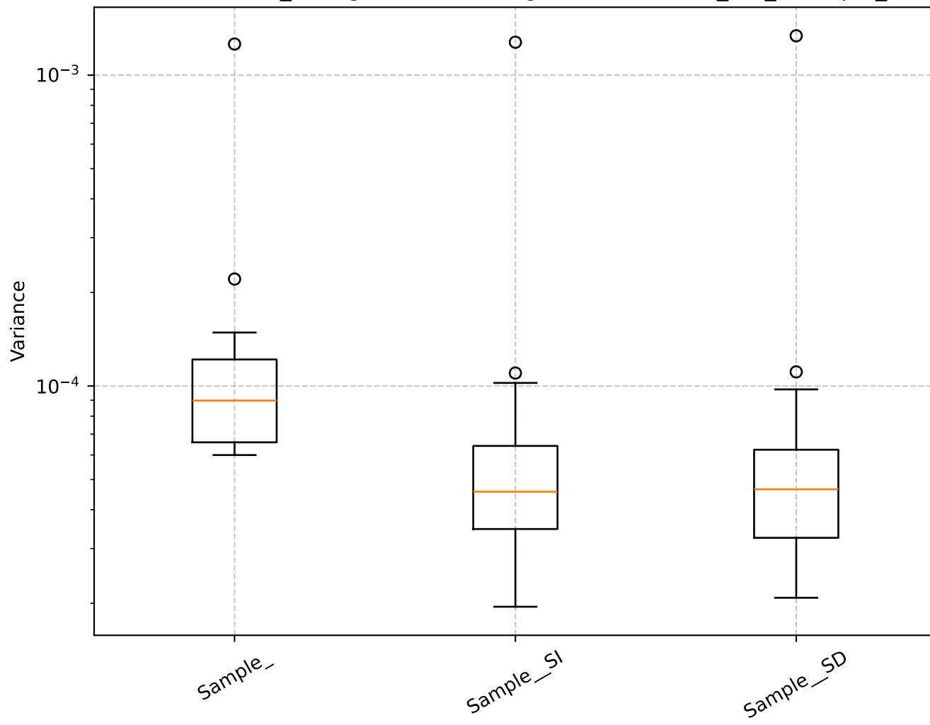
Q=0.52, len_rolling=100: Shrinkage Box Plot - min_var_, Sample_
