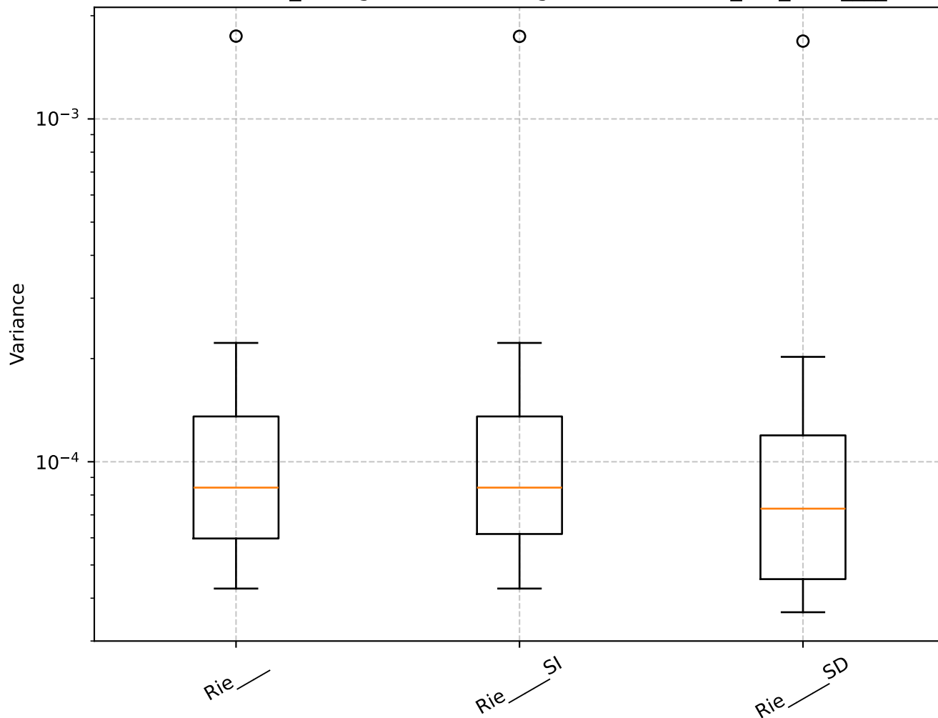
Q=0.53, len_rolling=100: Shrinkage Box Plot - min_var_, Rie____
