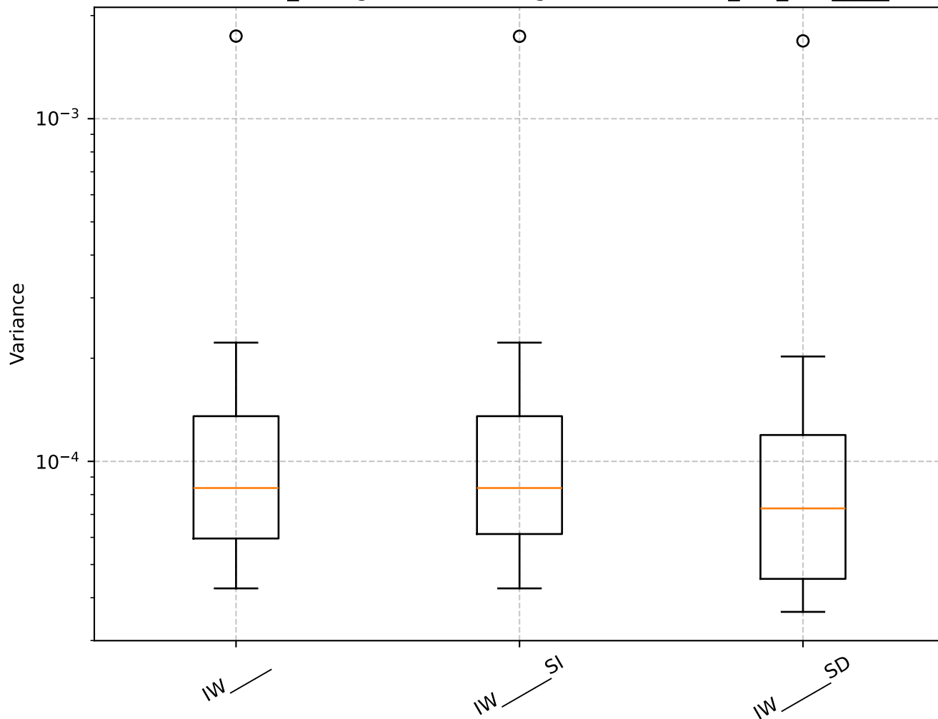
Q=0.55, len_rolling=100: Shrinkage Box Plot - min_var_, IW_____
