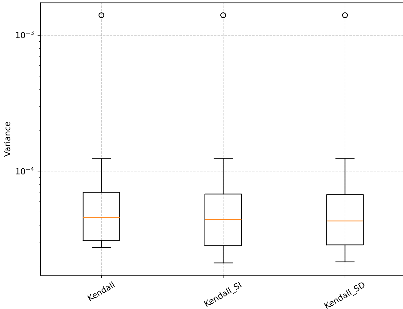
Q=0.56, len_rolling=100: Shrinkage Box Plot - min_var_, Kendall
