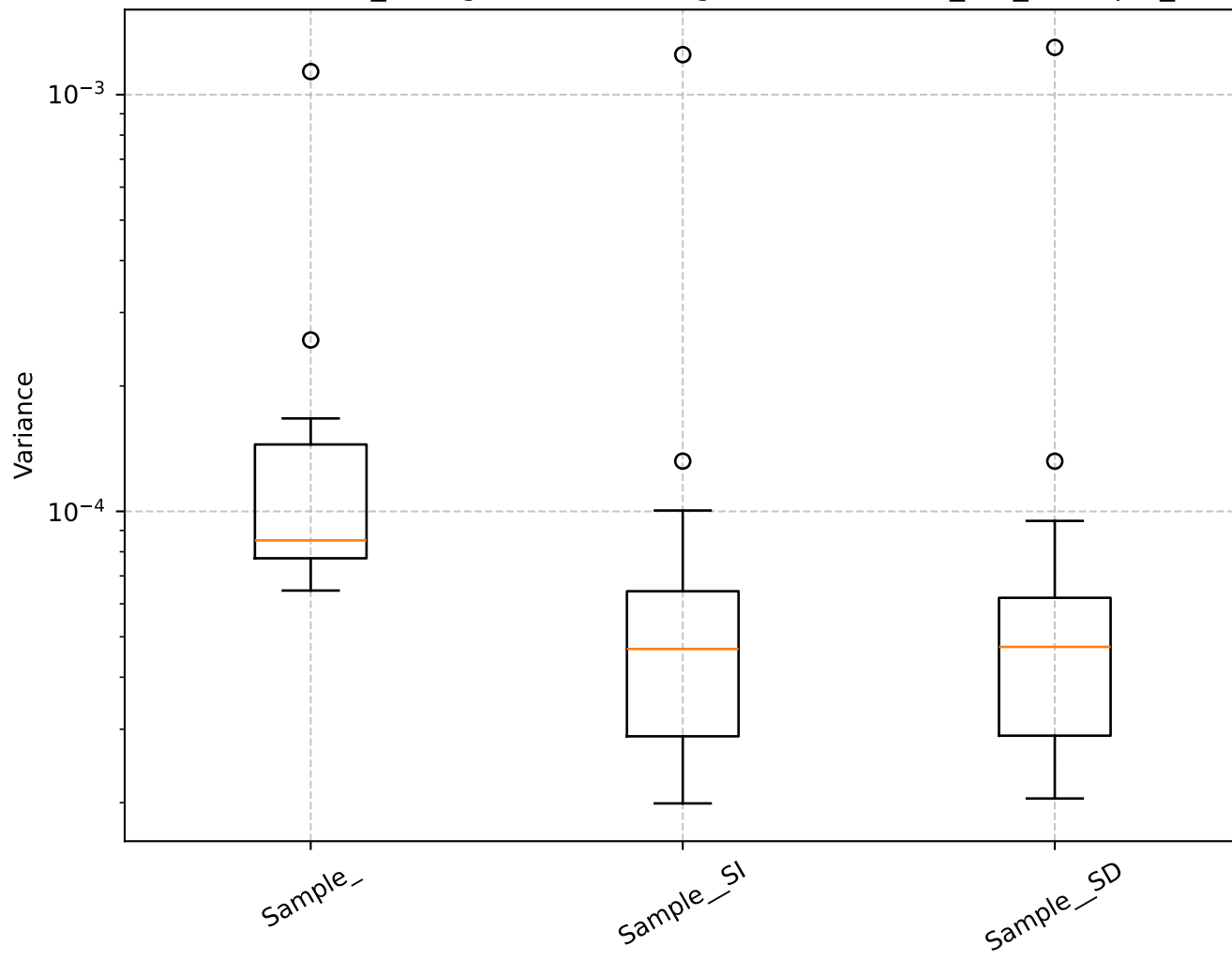
Q=0.56, len_rolling=100: Shrinkage Box Plot - min_var_, Sample_
