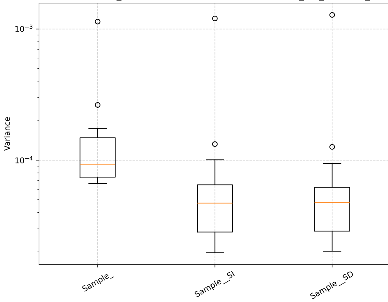
Q=0.57, len_rolling=100: Shrinkage Box Plot - min_var_, Sample_
