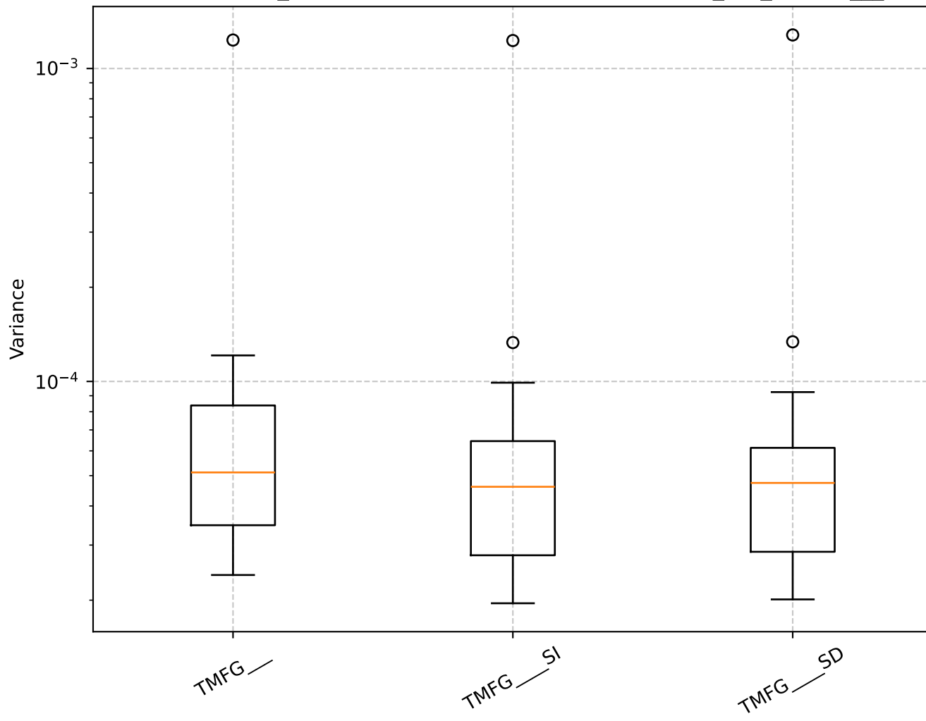
Q=0.58, len_rolling=100: Shrinkage Box Plot - min_var_, TMFG__
