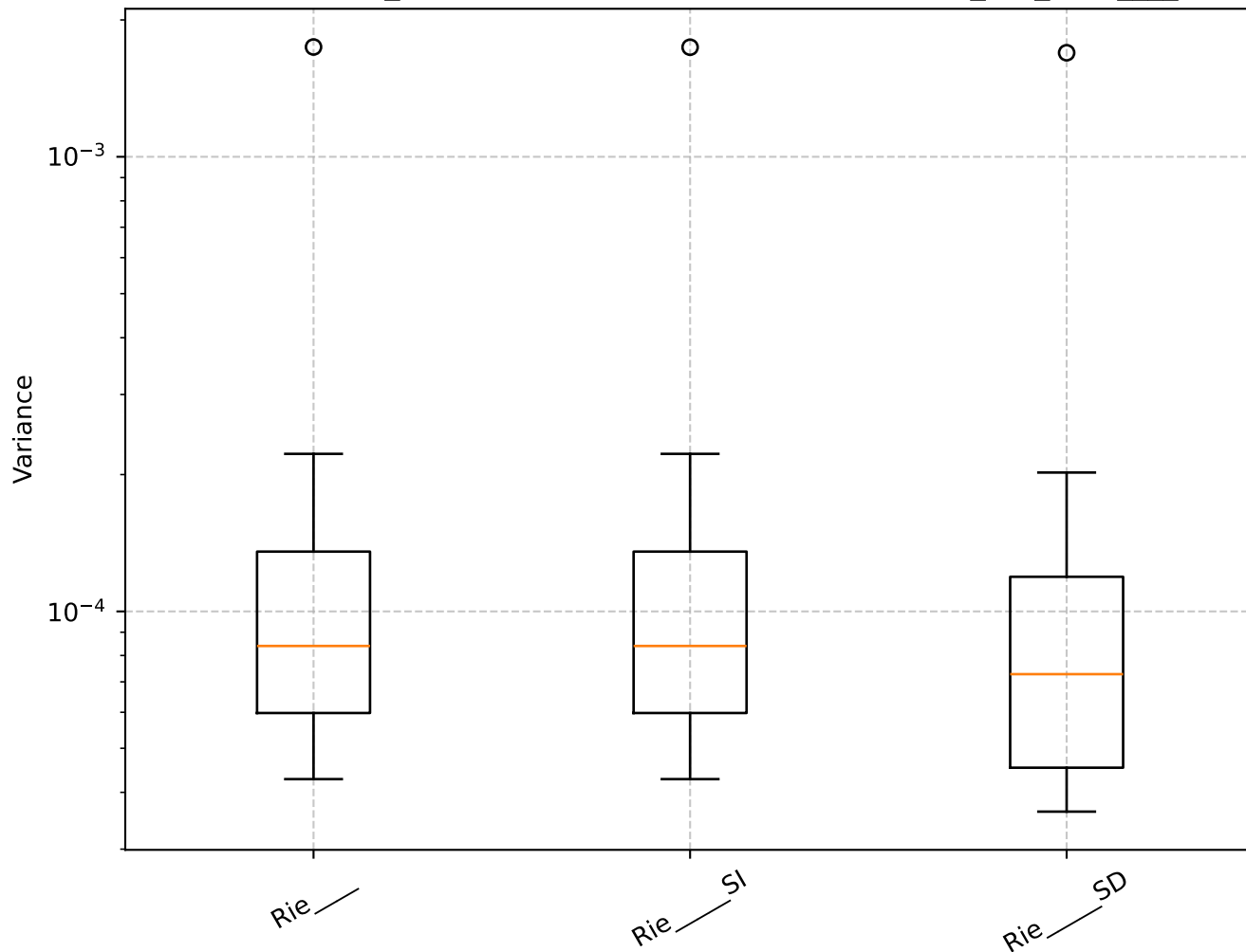
Q=0.59, len_rolling=100: Shrinkage Box Plot - min_var_, Rie____
