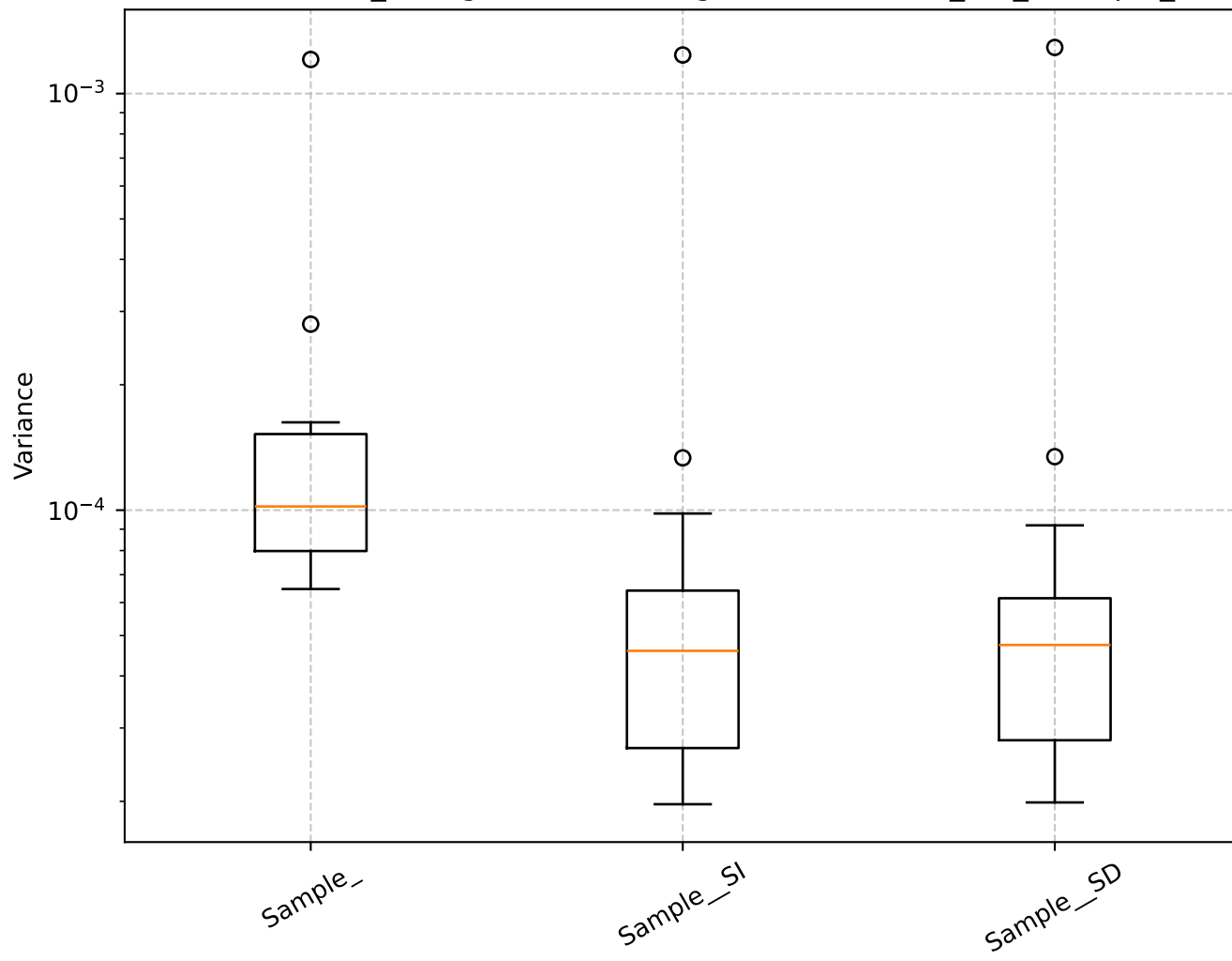
Q=0.59, len_rolling=100: Shrinkage Box Plot - min_var_, Sample_
