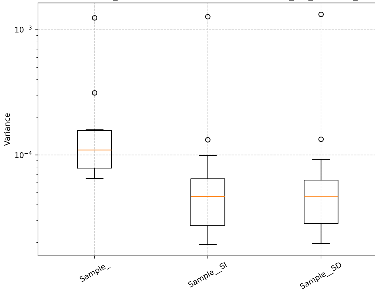
Q=0.62, len_rolling=100: Shrinkage Box Plot - min_var_, Sample_
