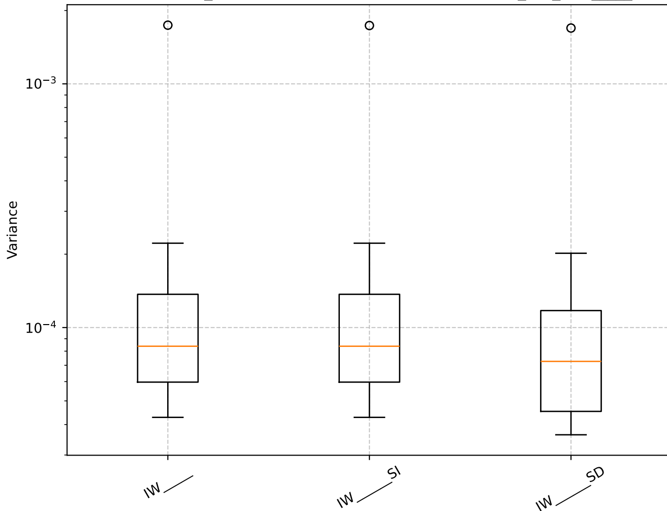
Q=0.65, len_rolling=100: Shrinkage Box Plot - min_var_, IW_____
