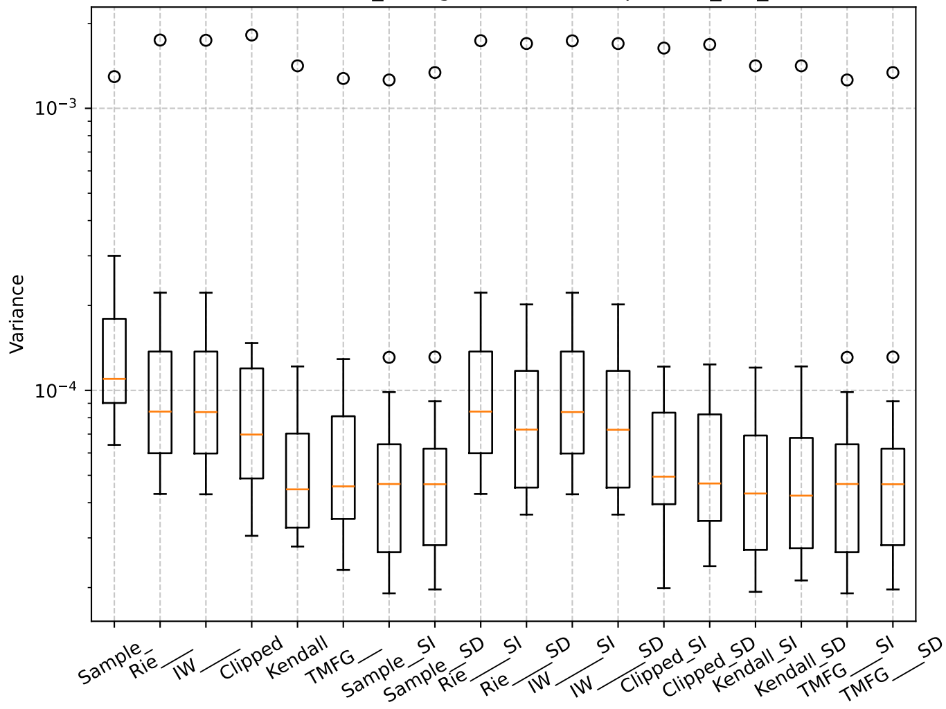
Q=0.66, len_rolling=100: Box Plot per min_var_
