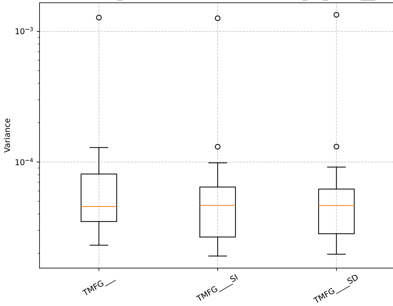
Q=0.66, len_rolling=100: Shrinkage Box Plot - min_var_, TMFG__
