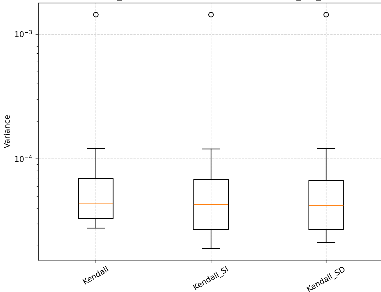
Q=0.67, len_rolling=100: Shrinkage Box Plot - min_var_, Kendall
