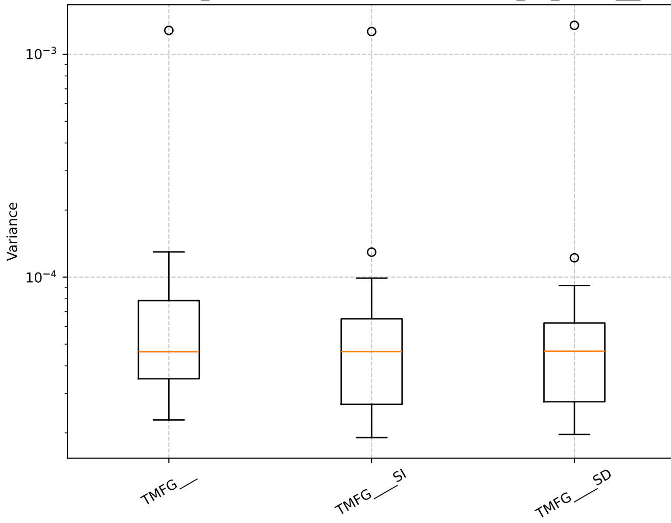
Q=0.67, len_rolling=100: Shrinkage Box Plot - min_var_, TMFG__
