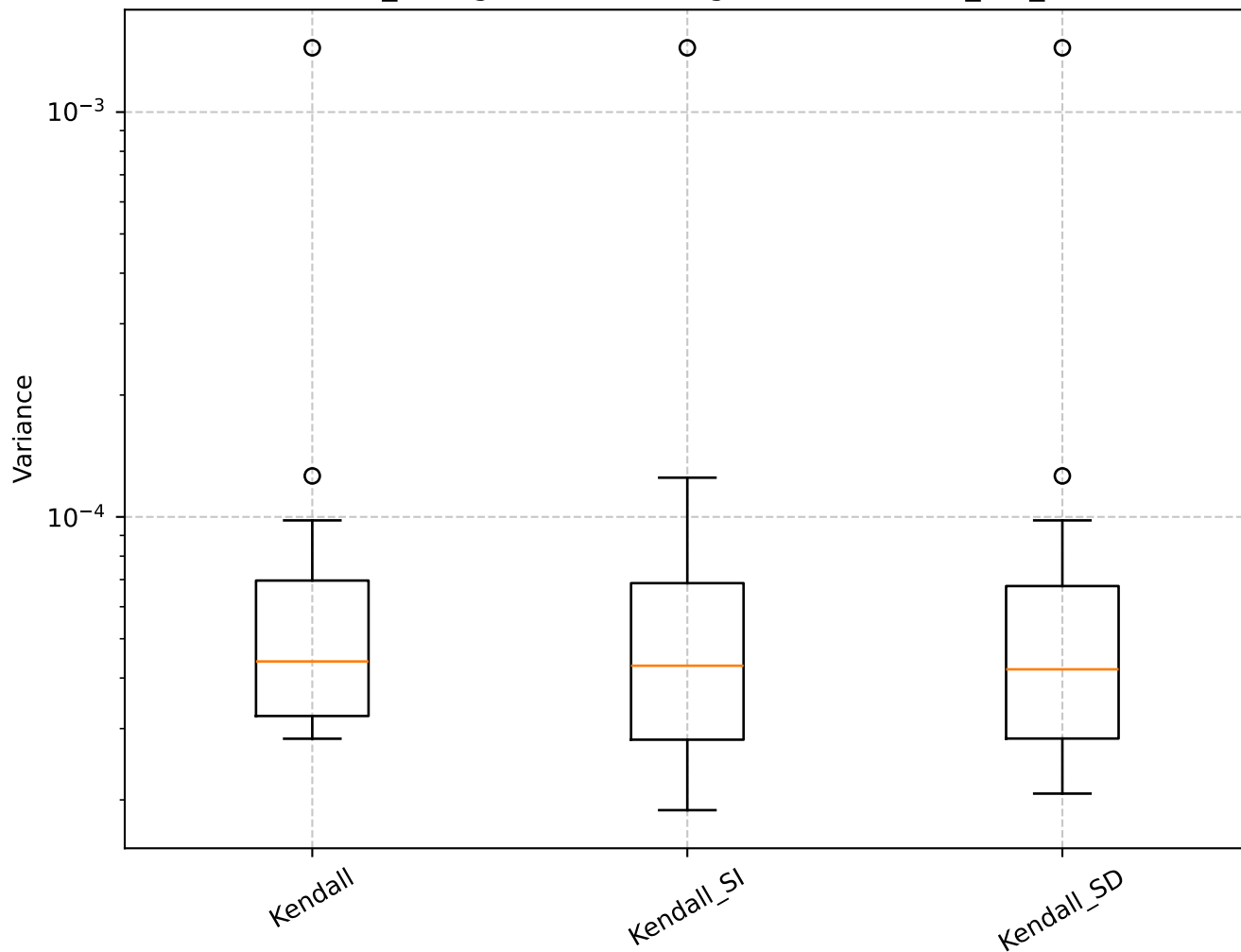
Q=0.71, len_rolling=100: Shrinkage Box Plot - min_var_, Kendall
