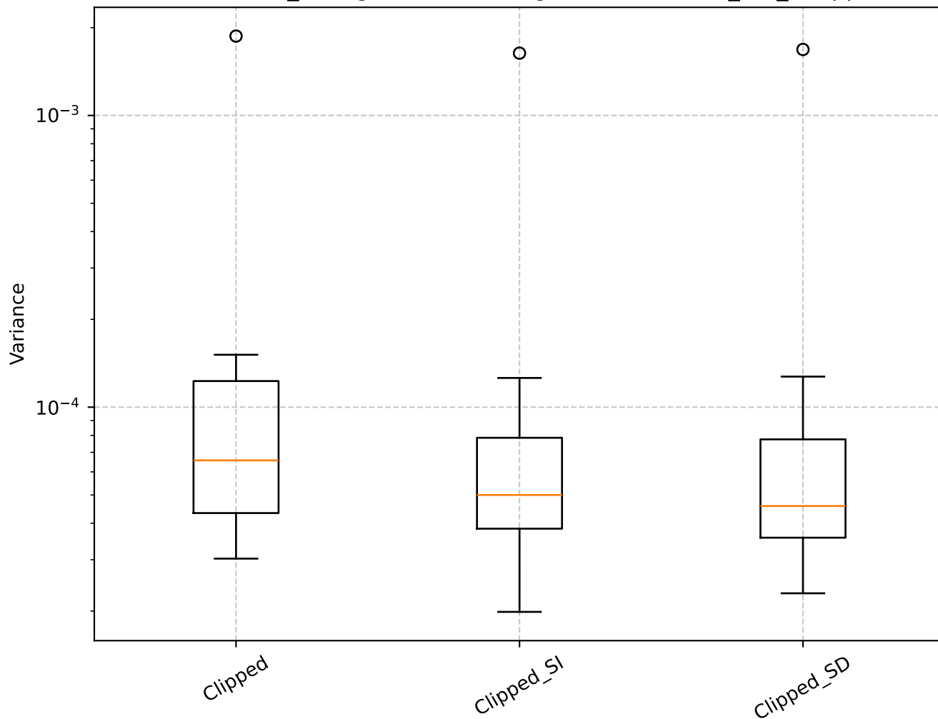
Q=0.75, len_rolling=100: Shrinkage Box Plot - min_var_, Clipped
