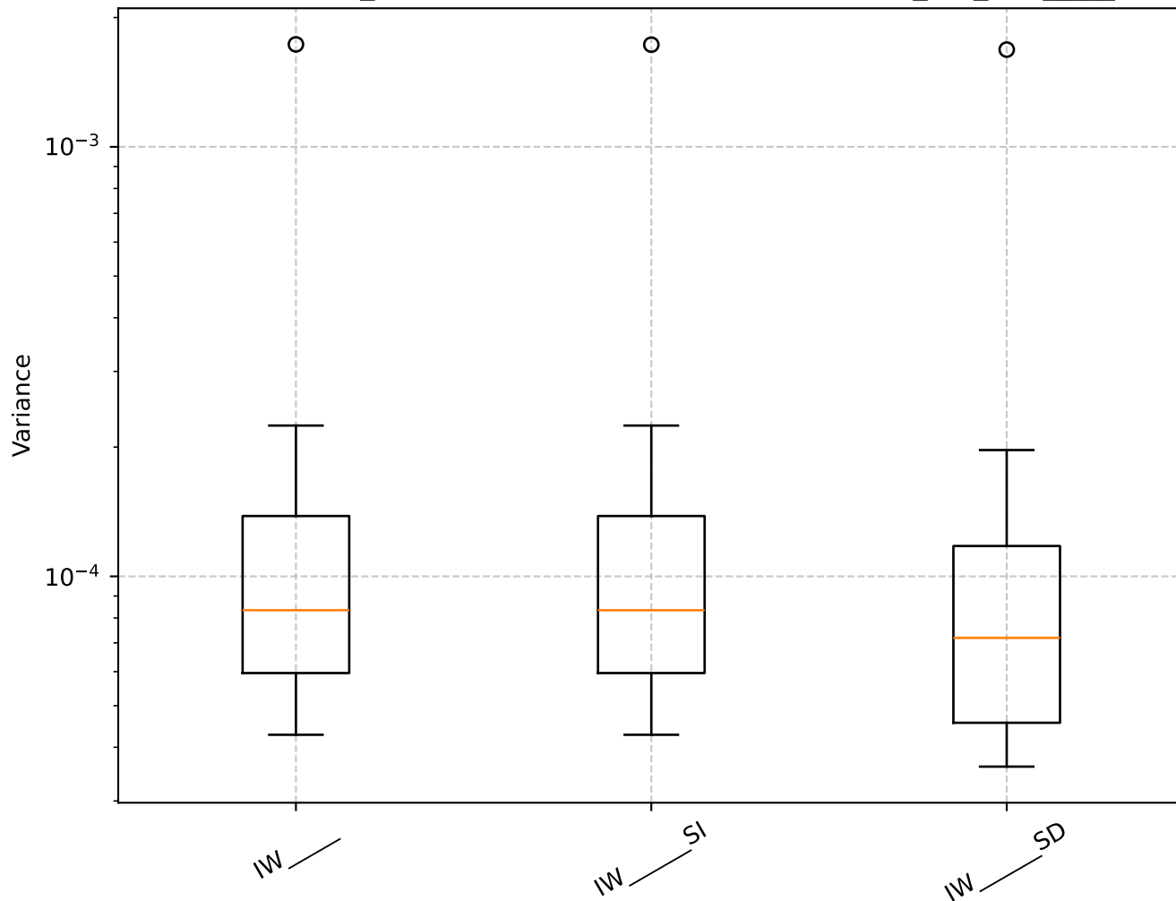
Q=0.78, len_rolling=100: Shrinkage Box Plot - min_var_, IW_____
