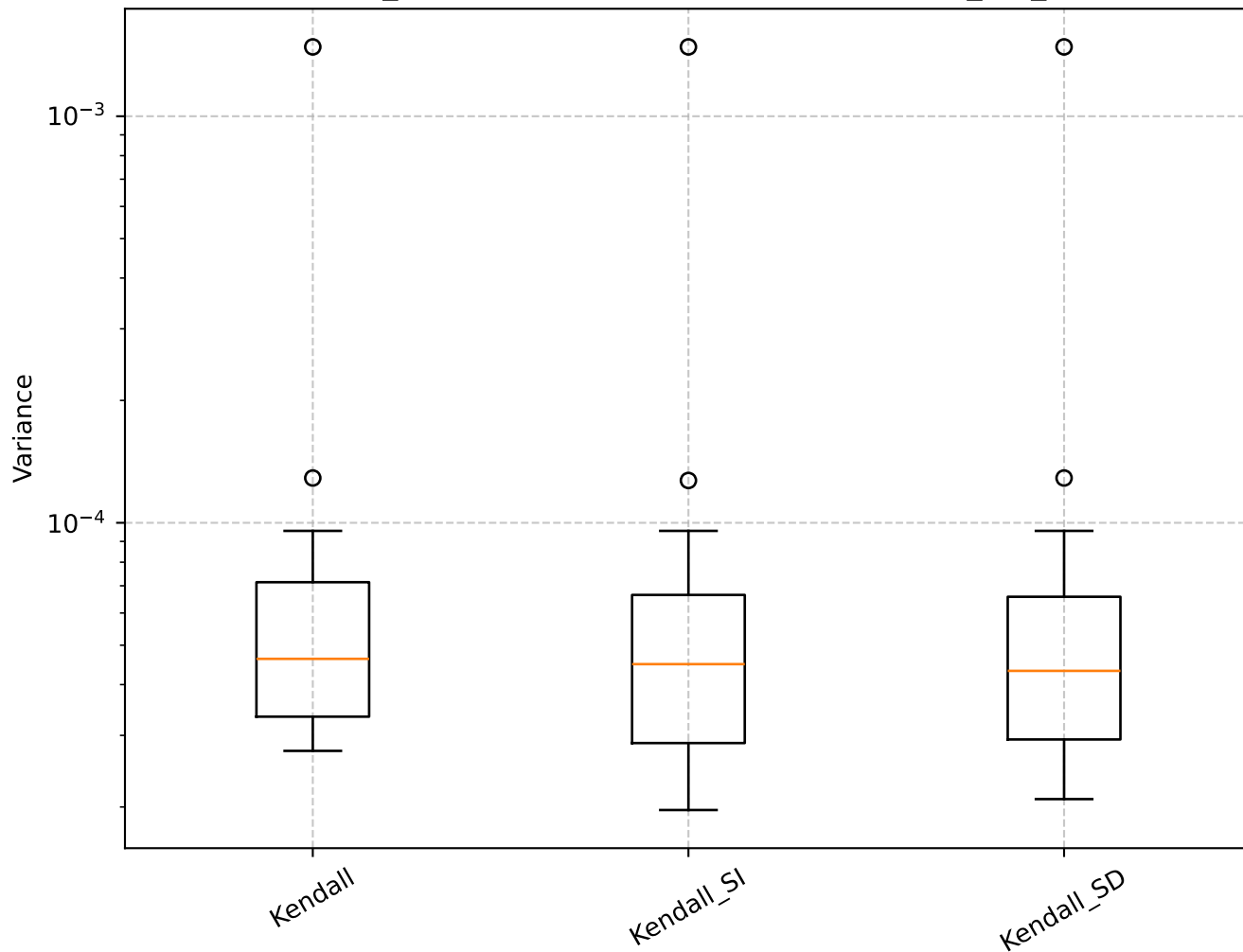
Q=0.78, len_rolling=100: Shrinkage Box Plot - min_var_, Kendall
