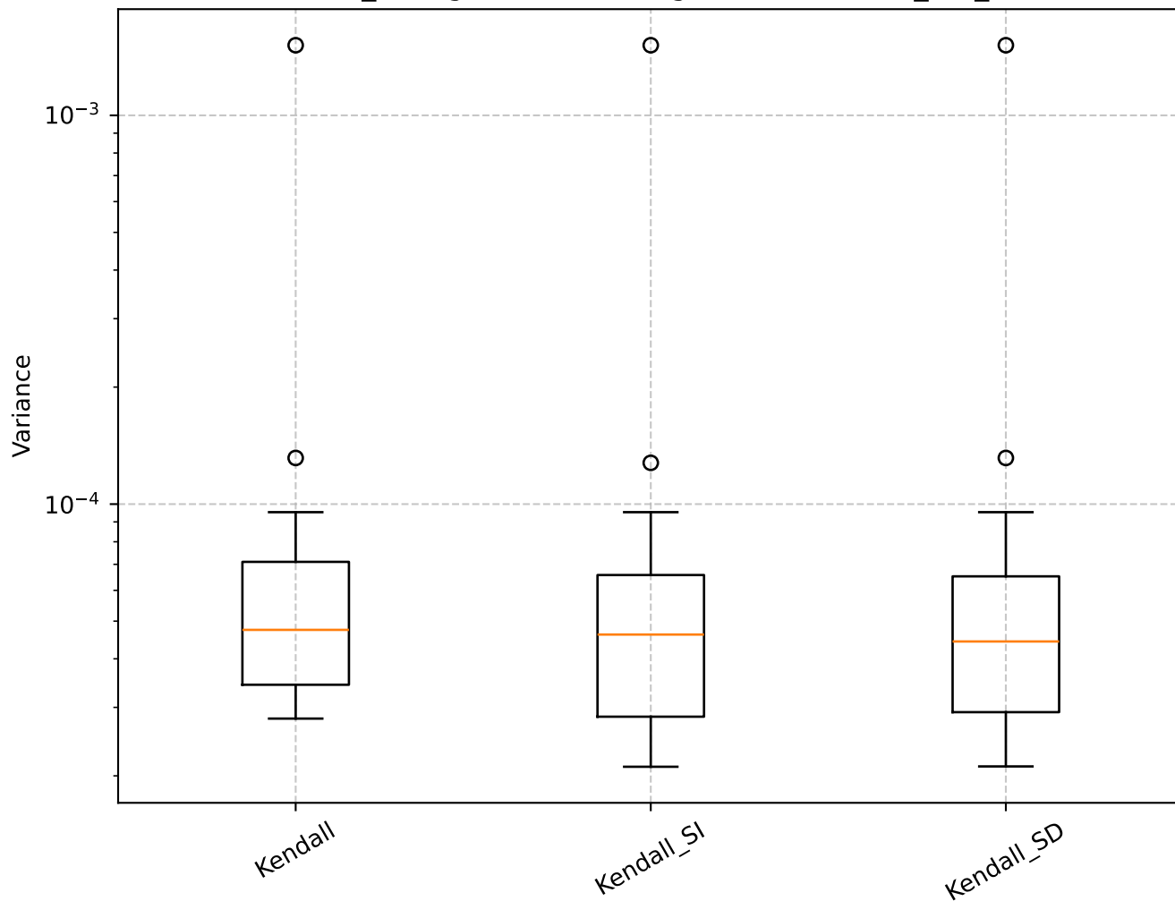
Q=0.83, len_rolling=100: Shrinkage Box Plot - min_var_, Kendall
