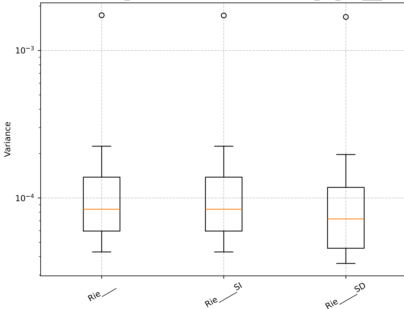
Q=0.83, len_rolling=100: Shrinkage Box Plot - min_var_, Rie____
