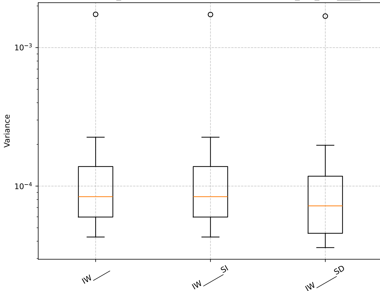
Q=0.85, len_rolling=100: Shrinkage Box Plot - min_var_, IW_____
