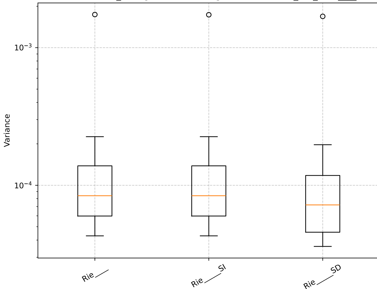
Q=0.85, len_rolling=100: Shrinkage Box Plot - min_var_, Rie____
