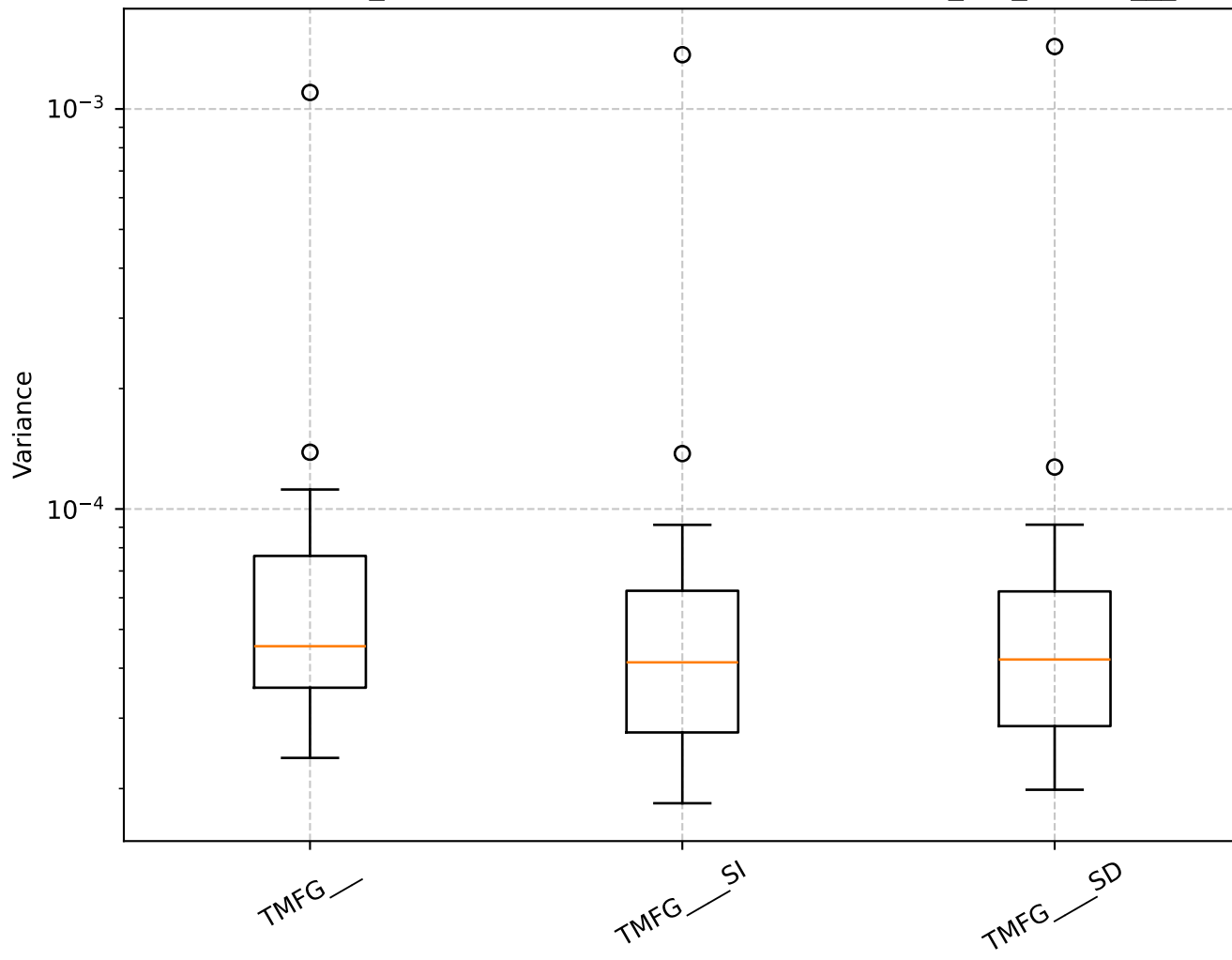
Q=0.85, len_rolling=100: Shrinkage Box Plot - min_var_, TMFG__
