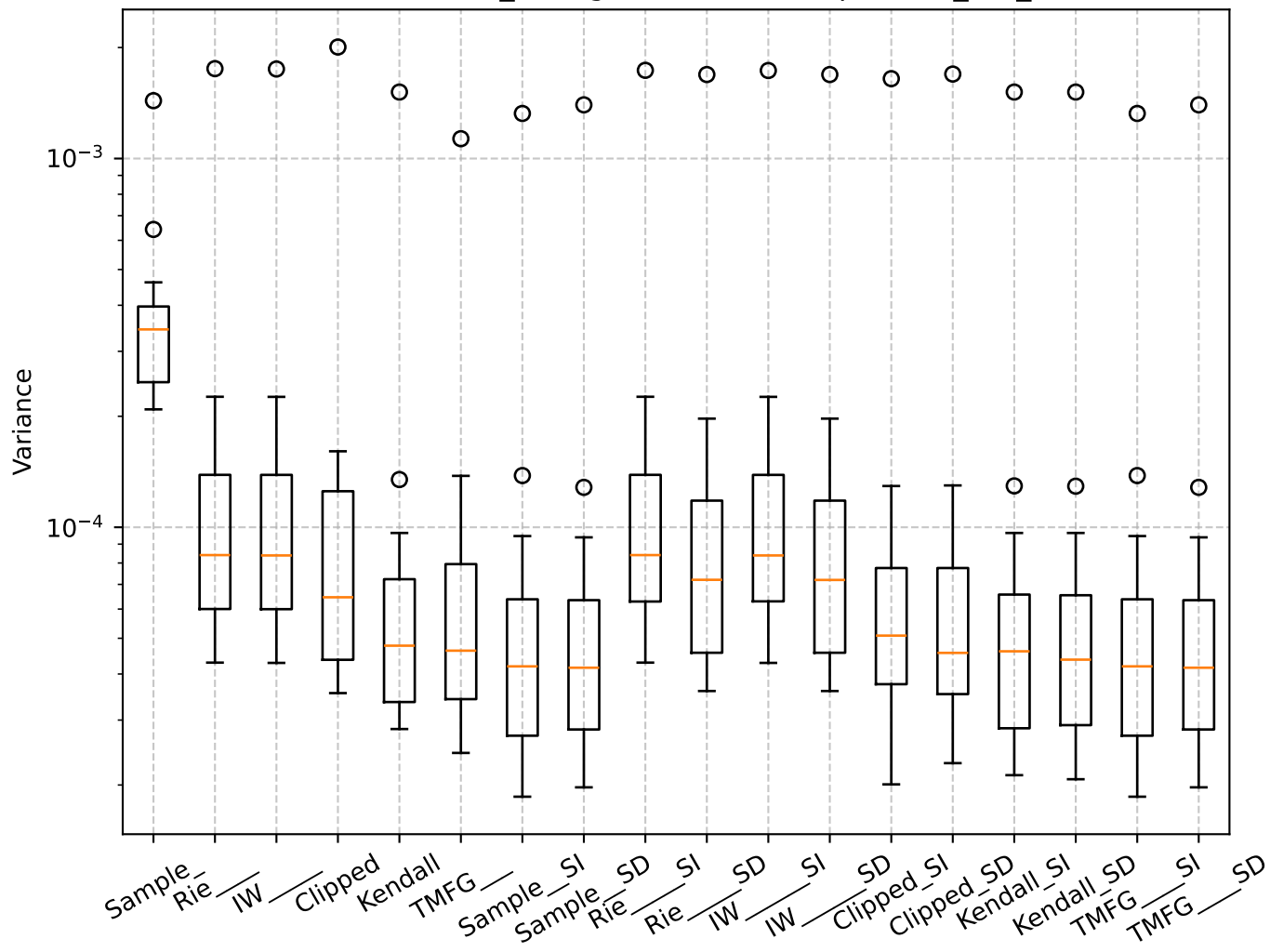
Q=0.87, len_rolling=100: Box Plot per min_var_
