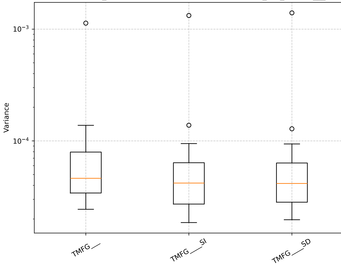
Q=0.87, len_rolling=100: Shrinkage Box Plot - min_var_, TMFG__
