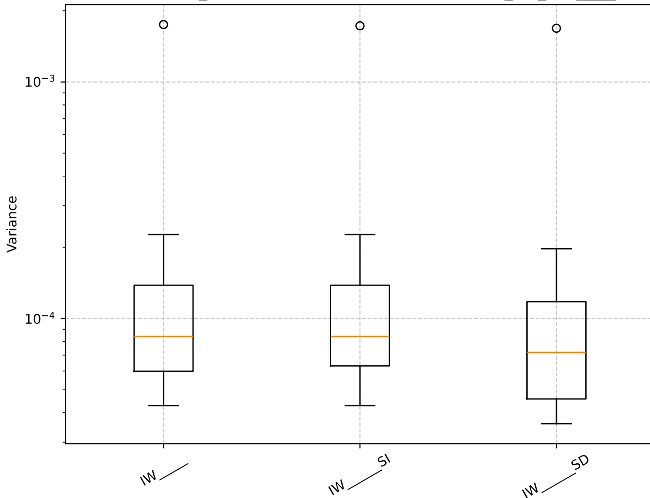
Q=0.91, len_rolling=100: Shrinkage Box Plot - min_var_, IW_____
