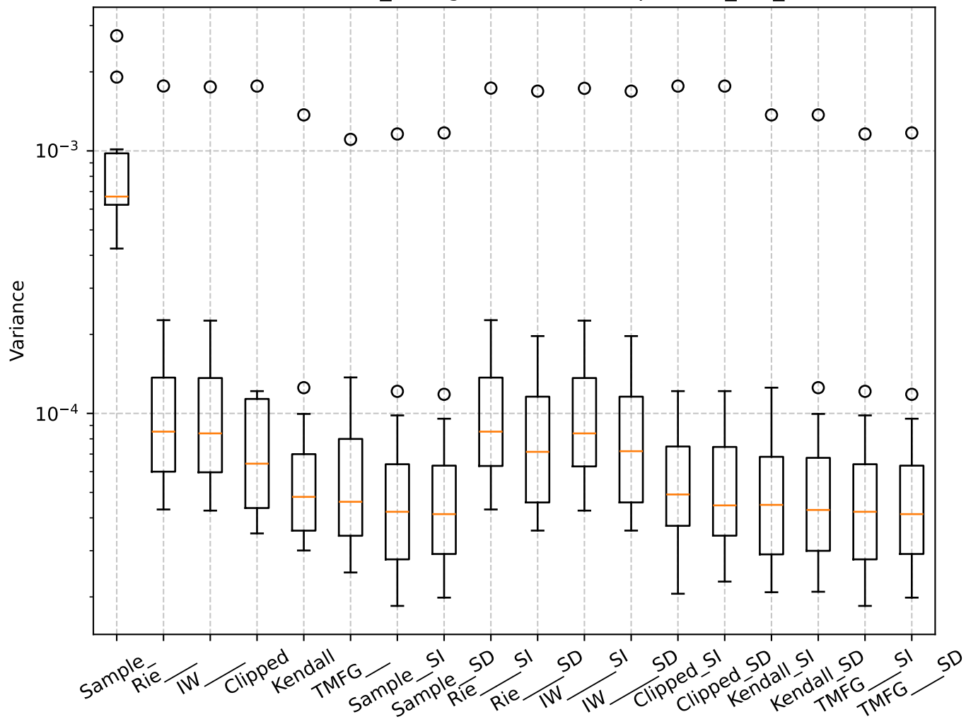
Q=0.95, len_rolling=100: Box Plot per min_var_
