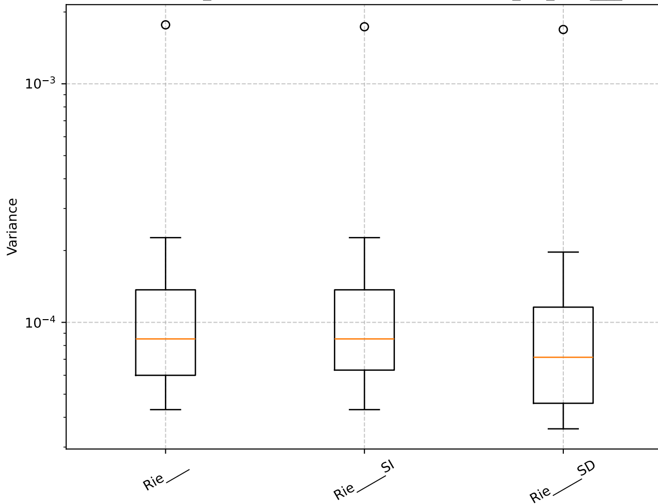
Q=0.95, len_rolling=100: Shrinkage Box Plot - min_var_, Rie____
