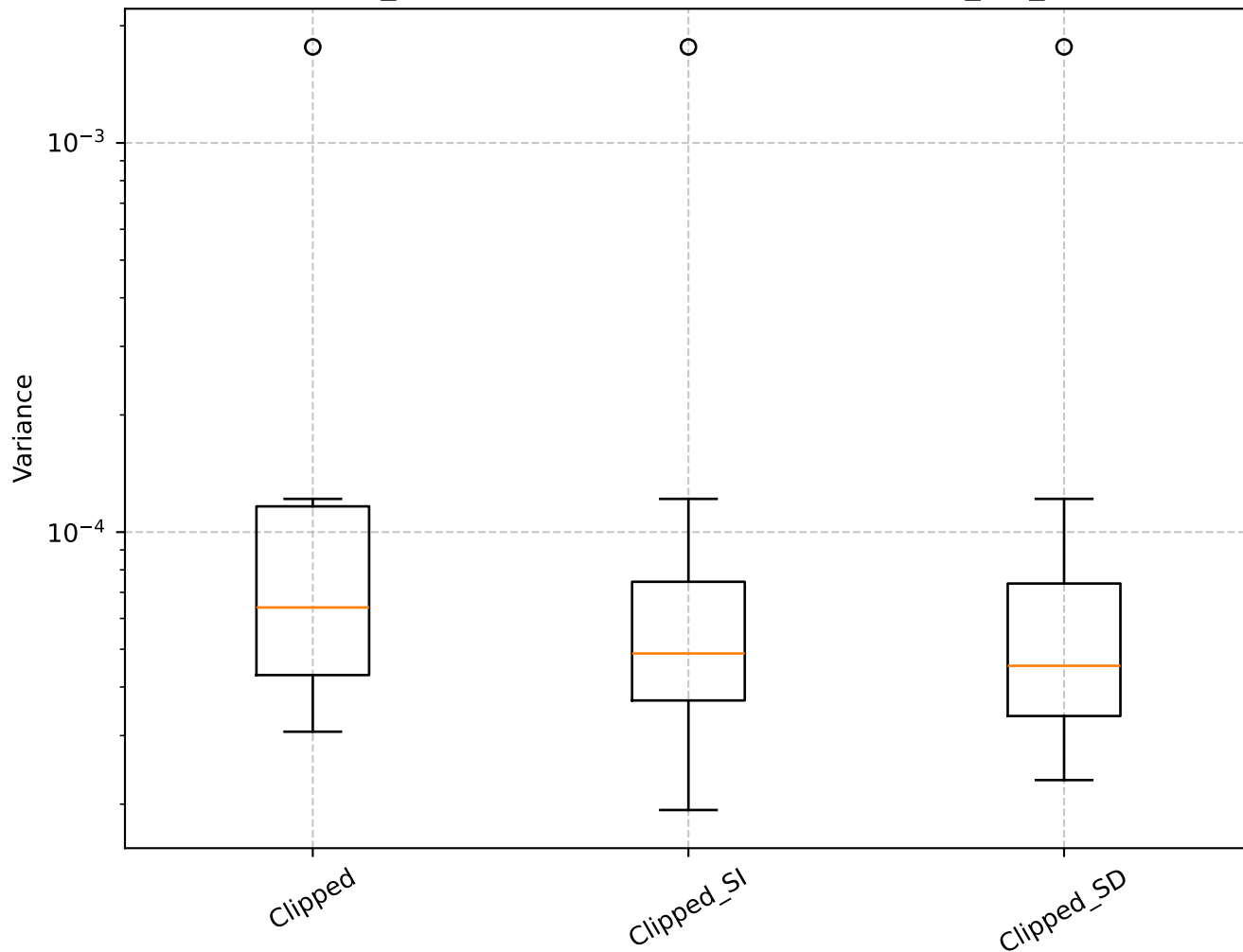
Q=1.03, len_rolling=100: Shrinkage Box Plot - min_var_, Clipped
