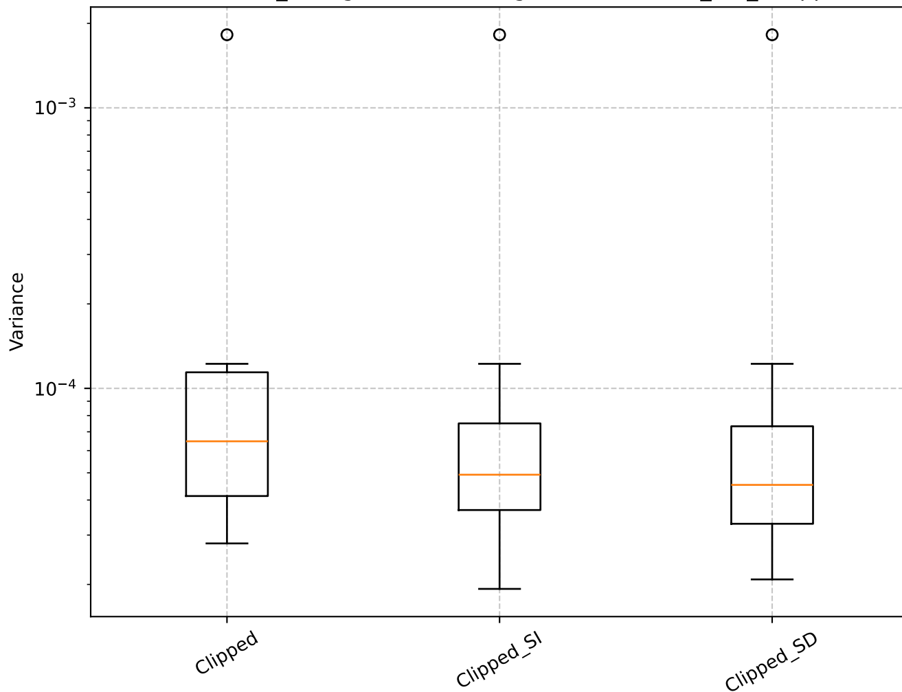
Q=1.05, len_rolling=100: Shrinkage Box Plot - min_var_, Clipped
