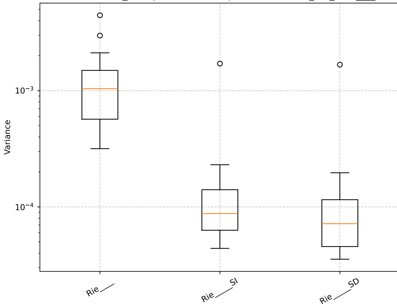
Q=1.05, len_rolling=100: Shrinkage Box Plot - min_var_, Rie____
