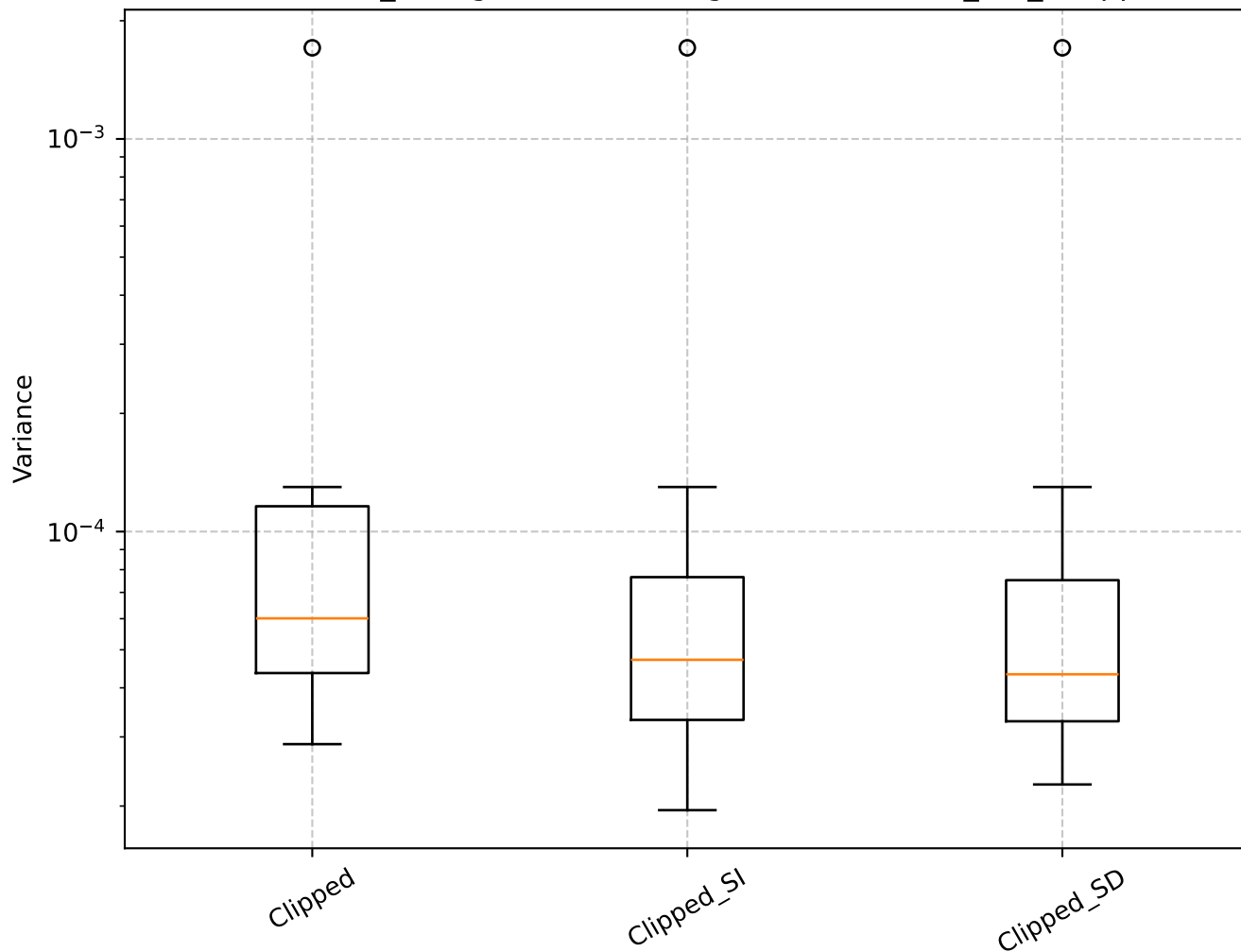
Q=1.21, len_rolling=100: Shrinkage Box Plot - min_var_, Clipped
