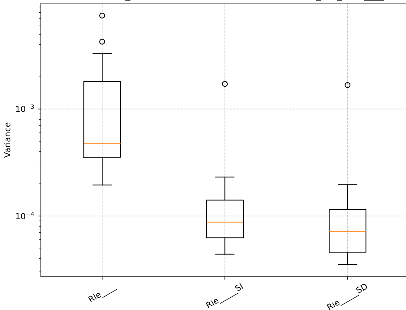
Q=1.21, len_rolling=100: Shrinkage Box Plot - min_var_, Rie_
