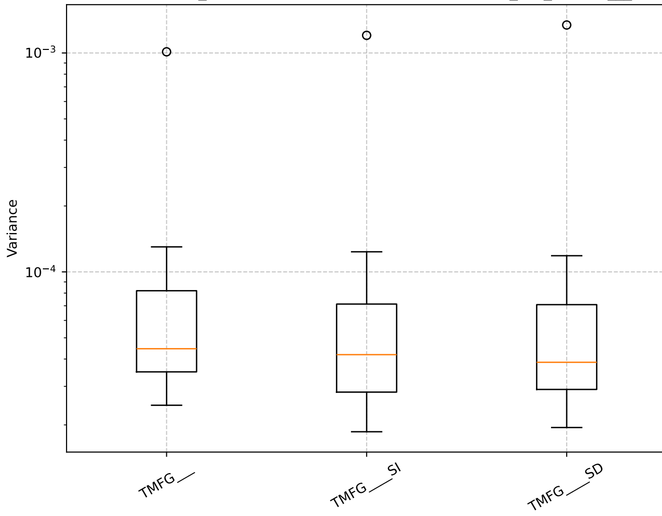
Q=1.21, len_rolling=100: Shrinkage Box Plot - min_var_, TMFG__
