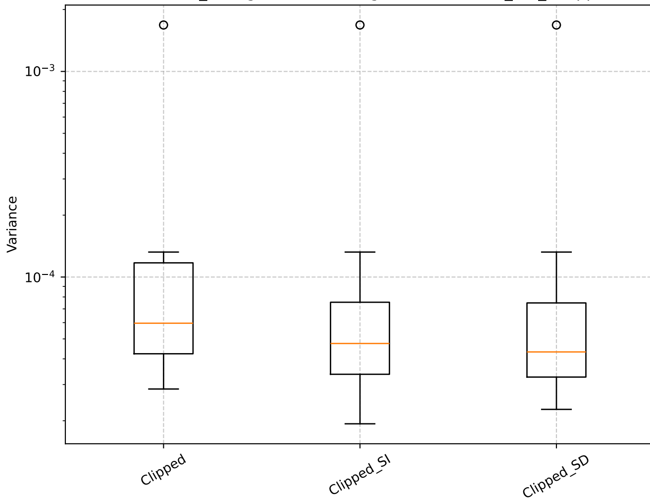
Q=1.25, len_rolling=100: Shrinkage Box Plot - min_var_, Clipped
