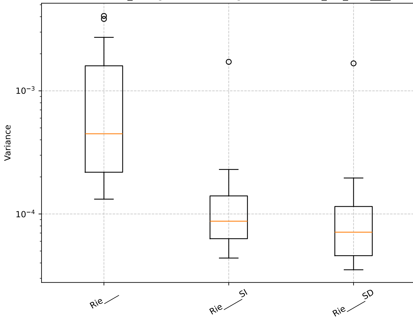
Q=1.29, len_rolling=100: Shrinkage Box Plot - min_var_, Rie____
