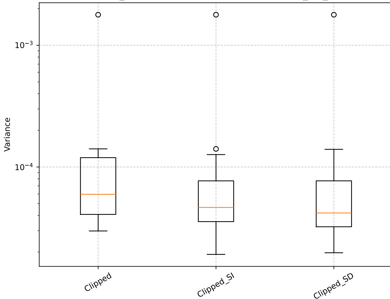
Q=1.38, len_rolling=100: Shrinkage Box Plot - min_var_, Clipped
