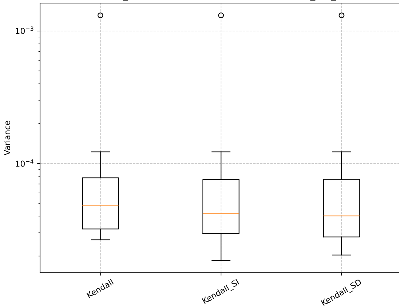
Q=1.38, len_rolling=100: Shrinkage Box Plot - min_var_, Kendall
