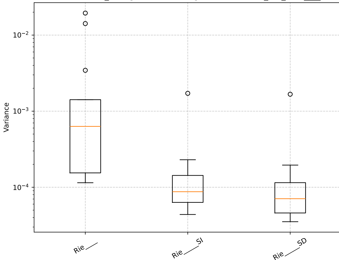
Q=1.38, len_rolling=100: Shrinkage Box Plot - min_var_, Rie____
