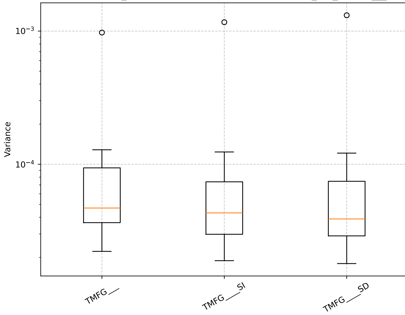
Q=1.43, len_rolling=100: Shrinkage Box Plot - min_var_, TMFG__
