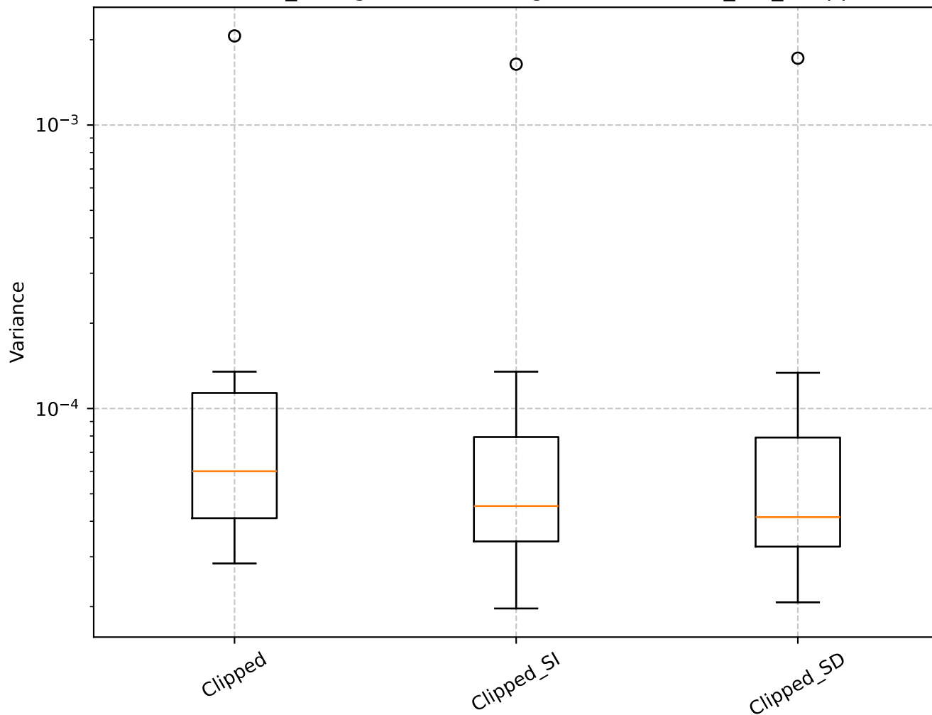
Q=1.48, len_rolling=100: Shrinkage Box Plot - min_var_, Clipped
