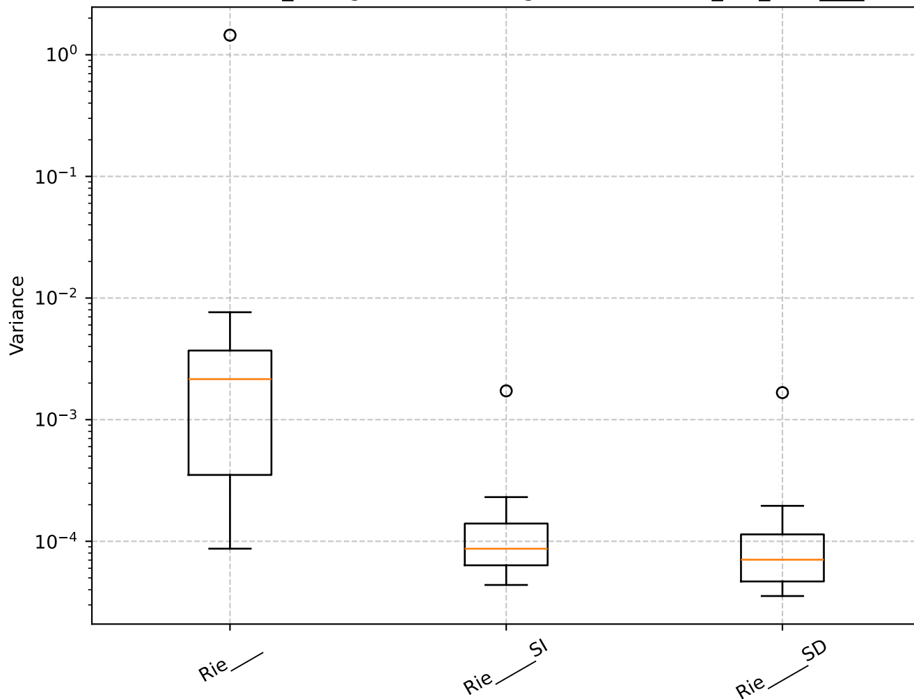
Q=1.67, len_rolling=100: Shrinkage Box Plot - min_var_, Rie____
