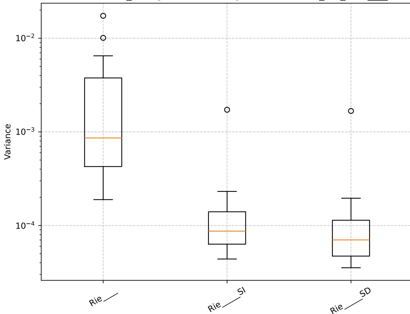
Q=1.75, len_rolling=100: Shrinkage Box Plot - min_var_, Rie____
