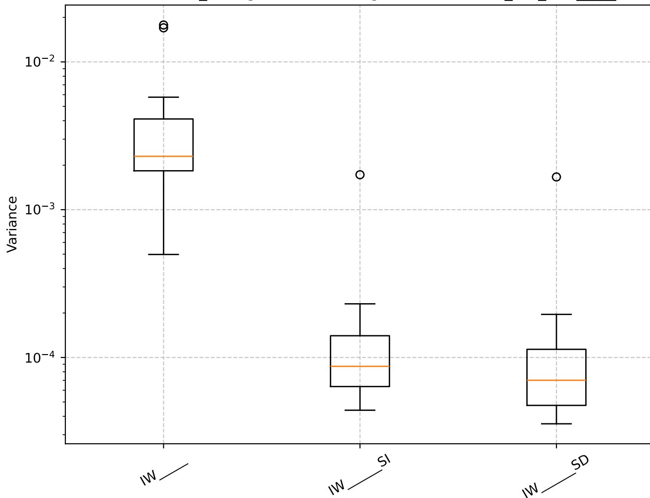
Q=1.83, len_rolling=100: Shrinkage Box Plot - min_var_, IW_____
