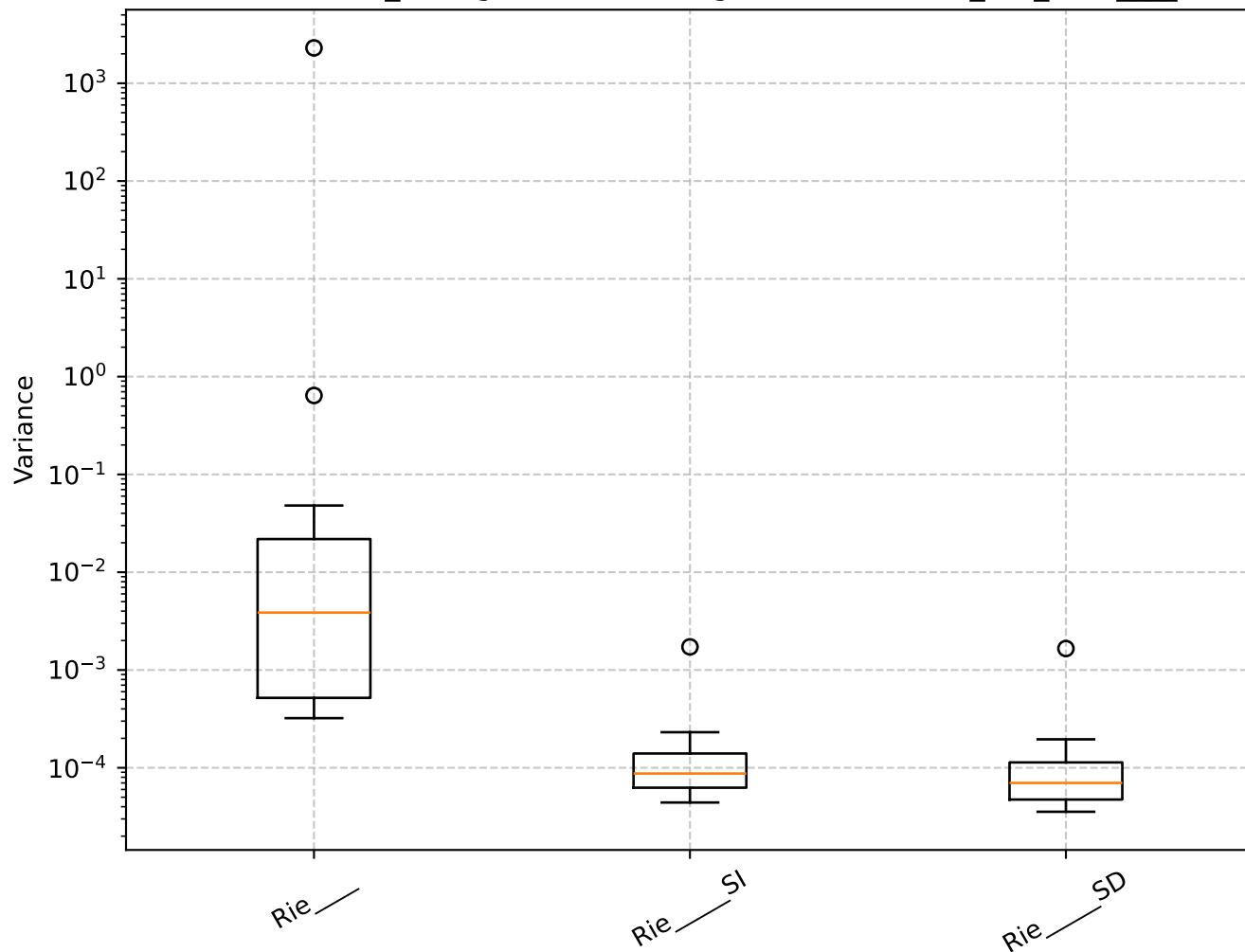
Q=1.90, len_rolling=100: Shrinkage Box Plot - min_var_, Rie____
