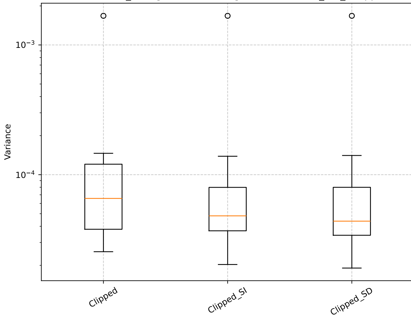
Q=2.00, len_rolling=100: Shrinkage Box Plot - min_var_, Clipped
