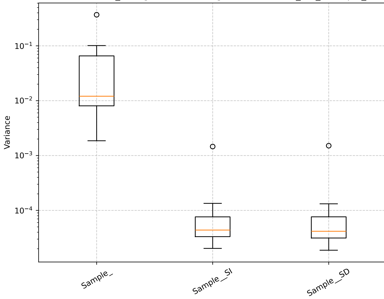
Q=2.00, len_rolling=100: Shrinkage Box Plot - min_var_, Sample_
