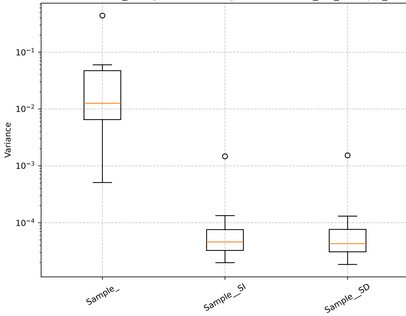
Q=2.12, len_rolling=100: Shrinkage Box Plot - min_var_, Sample_
